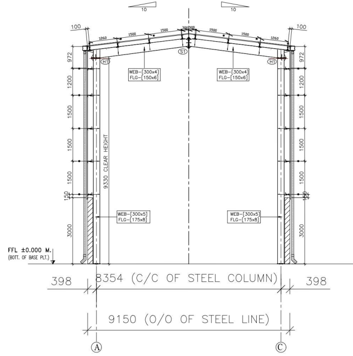
RIGID FRAME C/S ALONG GRID LINE 2 (* AS FLANGE BRACE BOTH SIDE)
