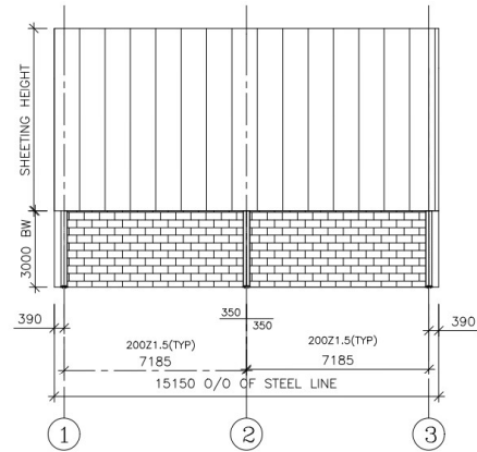
SHEETING ELEVATION ALONG GRID A
