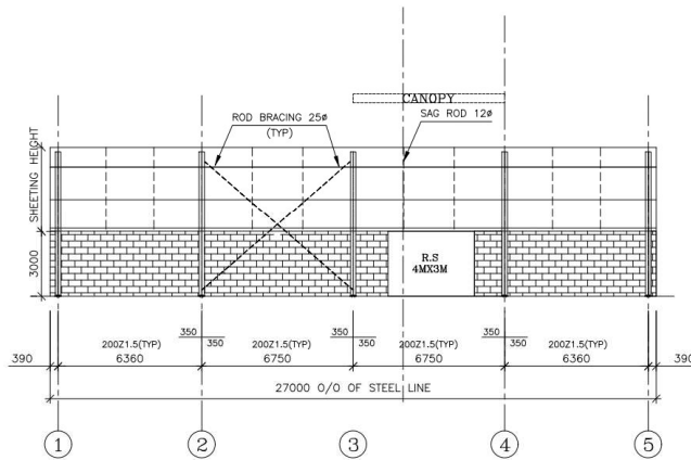
FRAMING ELEVATION ALONG GRID C ALL PURLIN/GIRTS 200 Z 1.5 (TYP)
