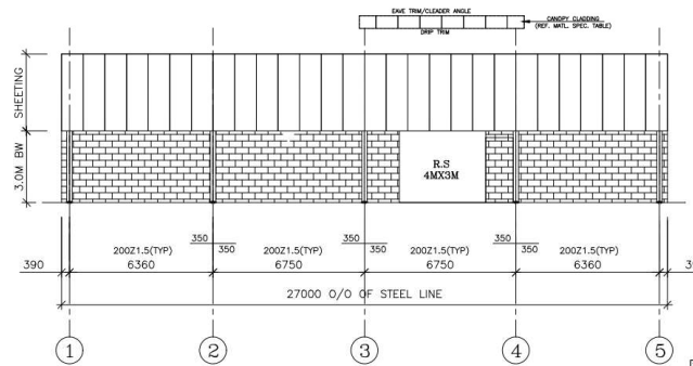
SHEETING ELEVATION ALONG GRID C
