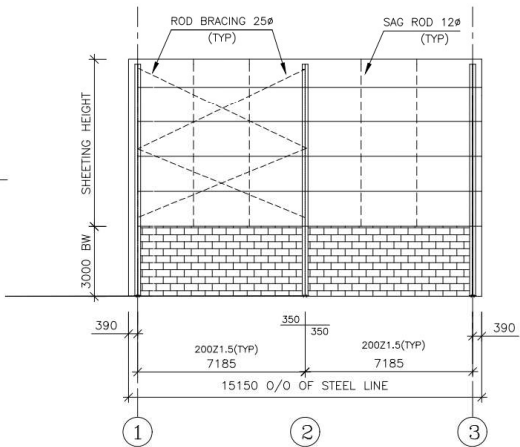
FRAMING ELEVATION ALONG GRID C ALL PURLIN/GIRTS 200 Z 1.5 (TYP)
