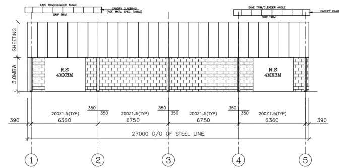
SHEETING ELEVATION ALONG GRID A
