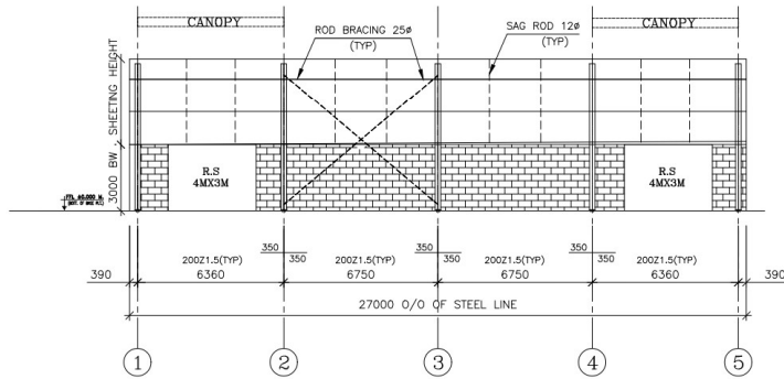
FRAMING ELEVATION ALONG GRID A ALL PURLIN/GIRTS 200 Z 1.5 (TYP)
