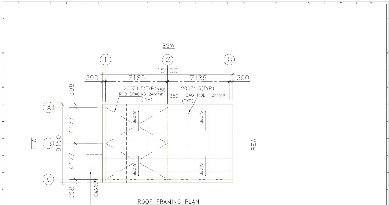
ROOF FRAMING PLAN
