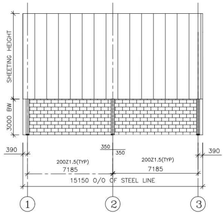
SHEETING ELEVATION ALONG GRID C
