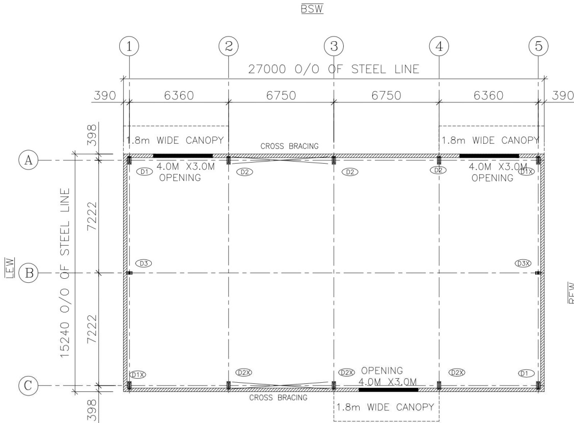
ANCHOR BOLT PLAN
