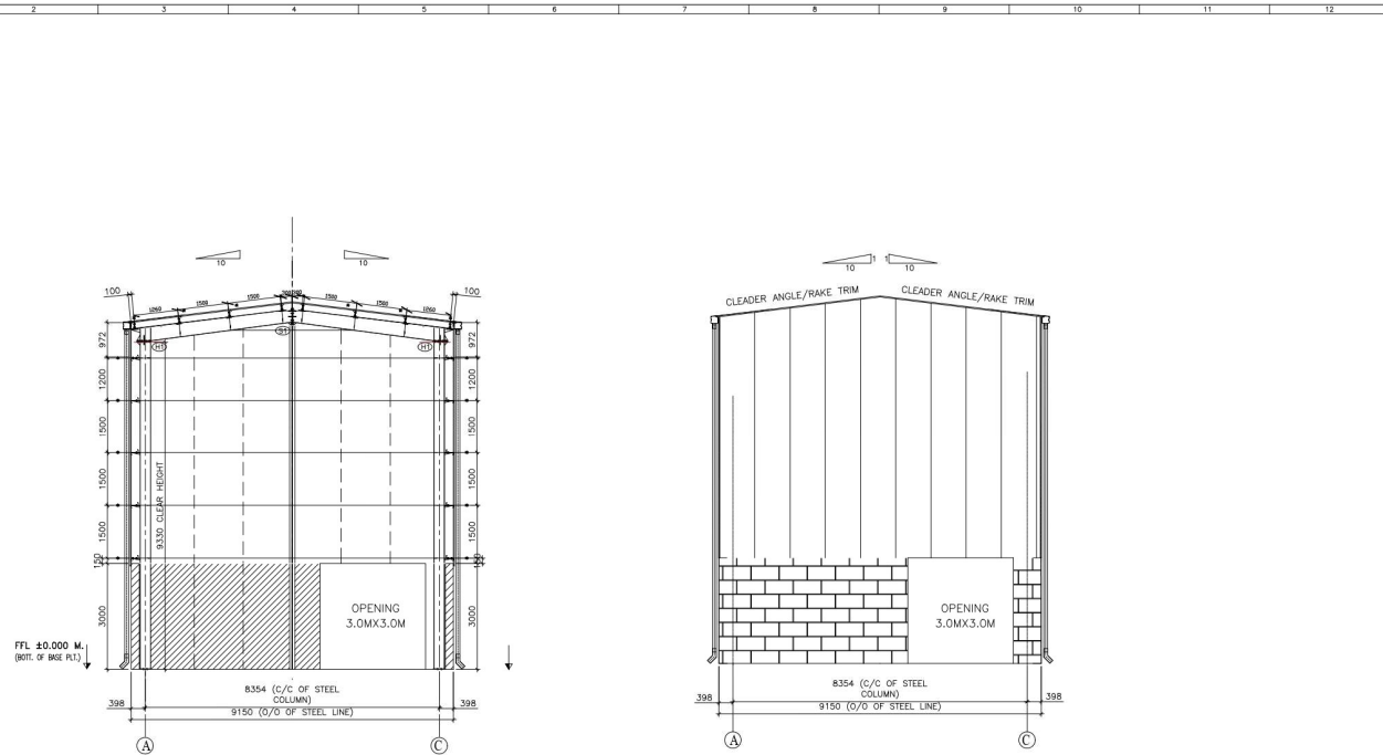
RIGID FRAME C/S ALONG GRID LINE-01 (* RAFTER AS FLANGE BRACE BOTH SIDE)
