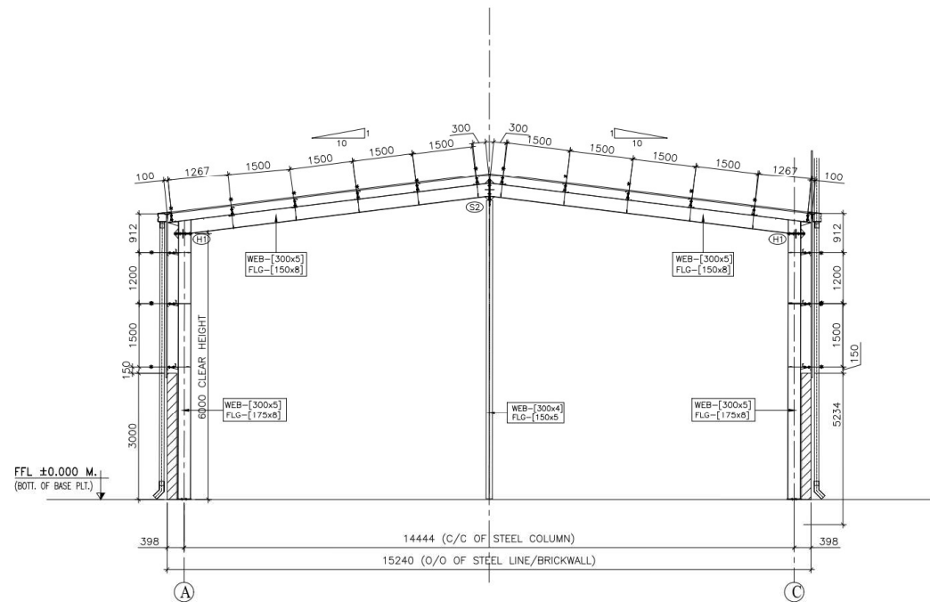
RIGID FRAME C/S ALONG GRID LINE-01&05 (* RAFTER AS FLANGE BRACE BOTH SIDE)
