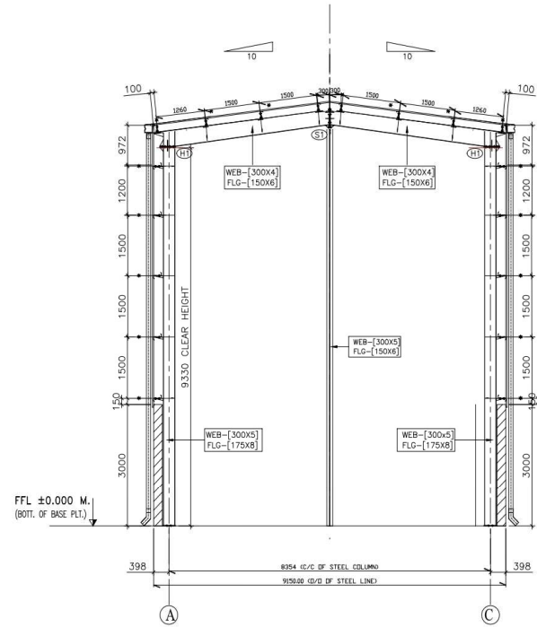
RIGID FRAME C/S ALONG GRID LINE-01&03 (* RAFTER AS FLANGE BRACE BOTH SIDE)
