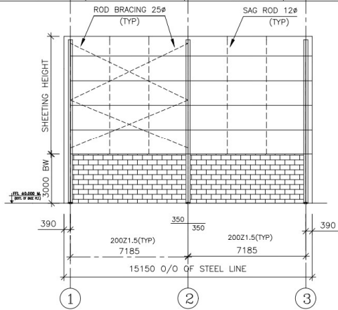
FRAMING ELEVATION ALONG GRID A ALL PURLIN/GIRTS 200 Z 1.5 (TYP)
